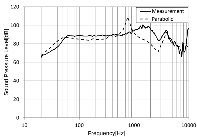
(c) Parabolic cone loudspeaker
