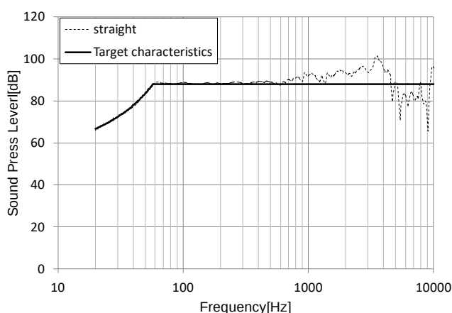
Fig.5 Objective function
