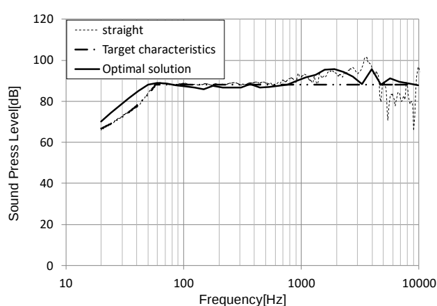
Fig. 6 Analysis result of optimal solution
