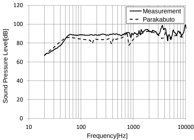
(a) Parakabuto cone loudspeaker
