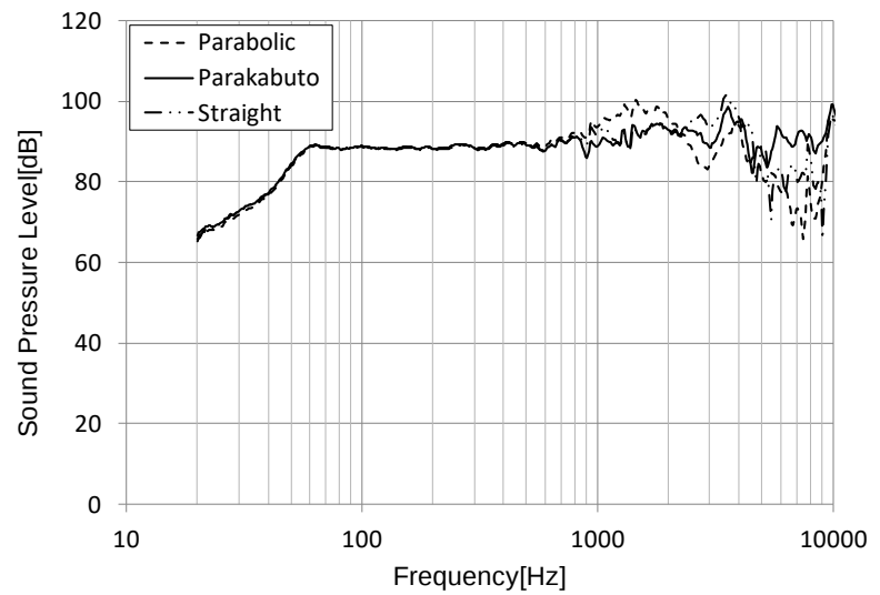
Fig.3 Measurement result of sound pressure frequency characteristics
